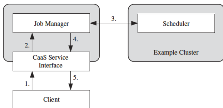
FIGURE 7.11. Job monitoring.
