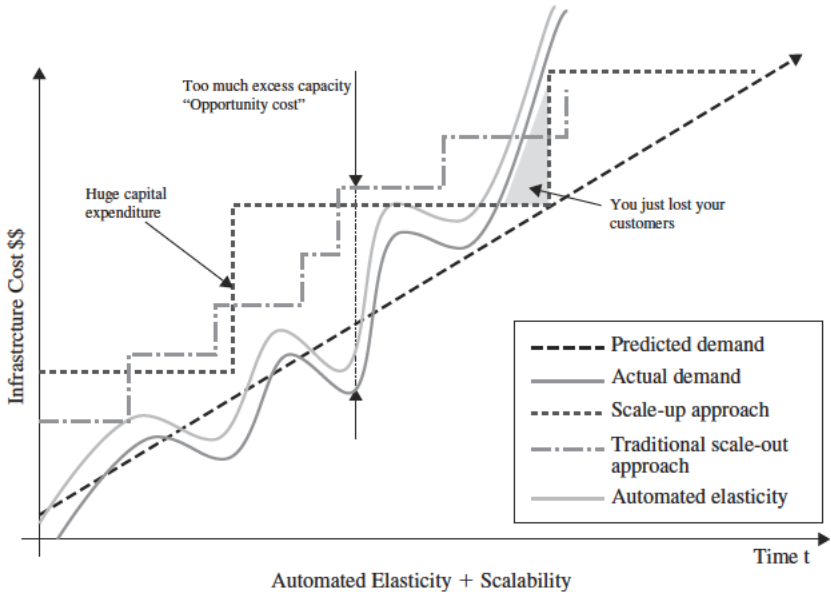
FIGURE 18.2. Automated elasticity.
