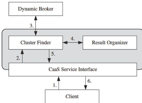
FIGURE 7.9. Cluster discovery.
